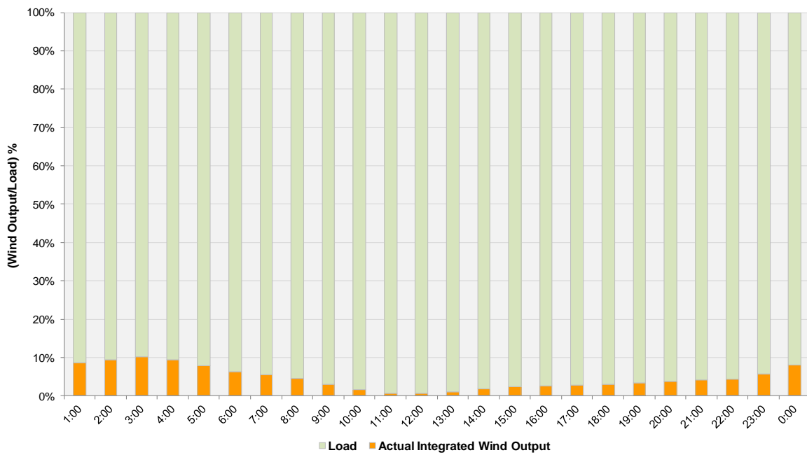
Actual Wind Output as a Percentage of the ERCOT Load 08-03-2011
