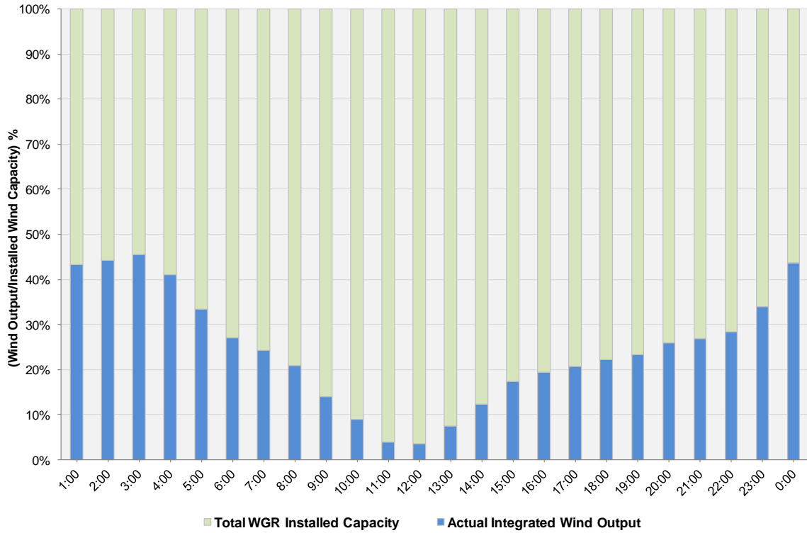
Actual Wind Output as a Percentage of the Total Installed Wind Capacity 08-03-2011
